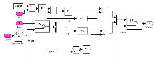
Fig. 5 Line side converter control for grid connected mode
