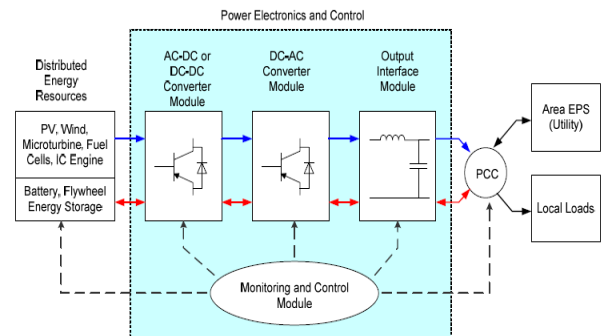
Fig. 1 Diagram of DE power electronics interface
