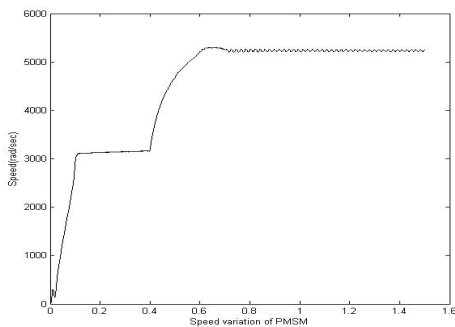
Fig. 7 Speed variation of PMSM
