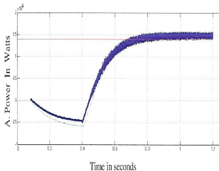
Fig. 8 Variation of active power starting/generating PMSM-side(14kW)
