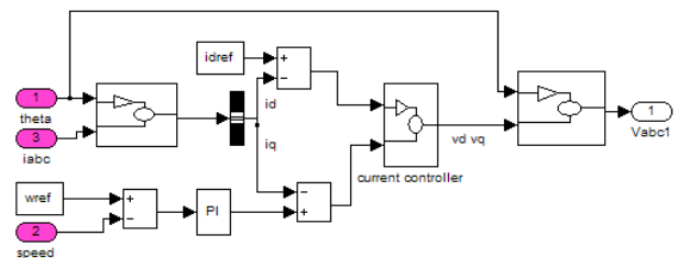
Fig. 4 Machine side converter control.
