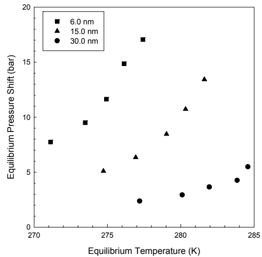
Fig. 5 Equilibrium pressure shifts between pore and bulk ethane hydrates
