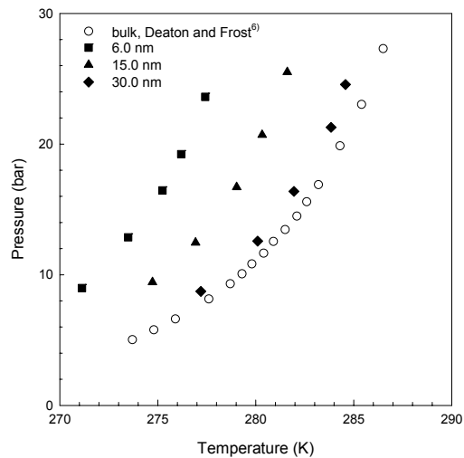
Fig. 4 Hydrate phase equilibria of the binary ethane + water mixtures in silicagel pores
