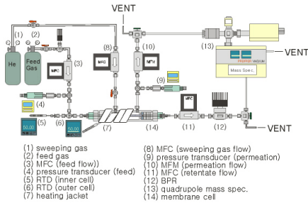
Fig. 1. Schematic diagram of membrane cell
