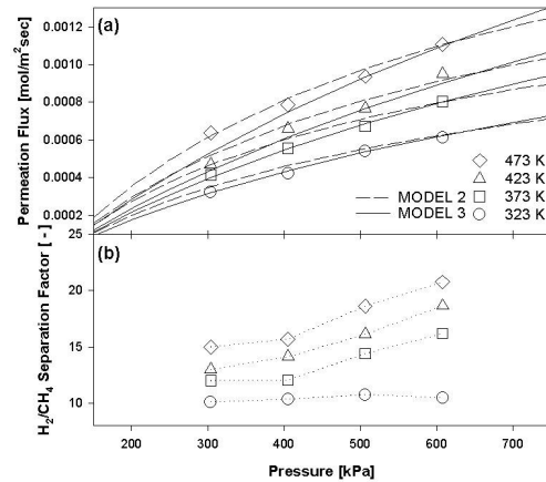
Fig. 4. Steady state permeation of H 2 /CH 4 binary mixture (50/50 v/v%) on MTES membrane at 323-473 K: (a) permeation flux and (b) H 2 /CH 4 separation factor : sweeping gas flow rate (=50 sccm) and stage cut (=0.60) were held constant [3].
