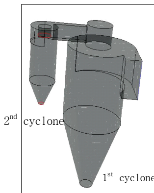
Fig. 1 Cyclone used in this work
