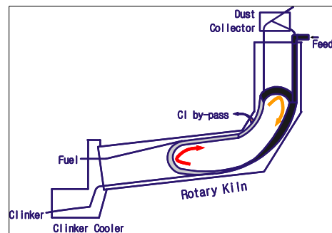
Fig. 2 Circulation characteristics of particle in kiln
