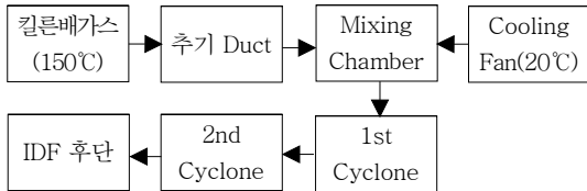
Fig. 3 Chlorine control unit in cement Manufacturing Process
