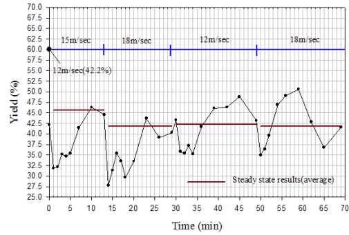
Fig. 4 Dynamic simulation for 1st cyclone
