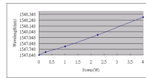
Fig. 3. Measured wavelength is function of the active power.
