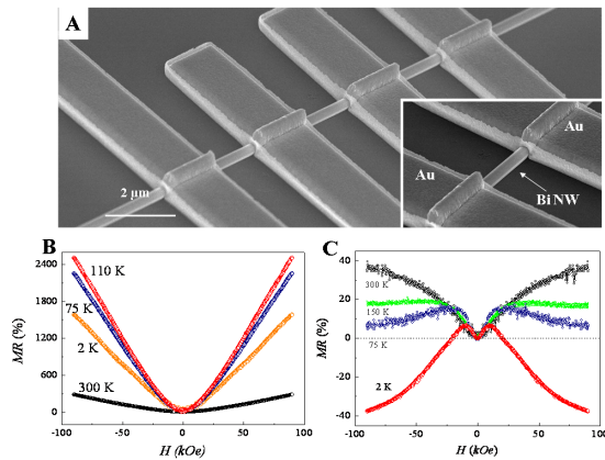
Fig. 1. (A) A SEM image of an individual Bi nanowire device. The OMR of the 400-nm-diameter Bi nanowire: (B) transverse and (C) longitudinal geometry.
