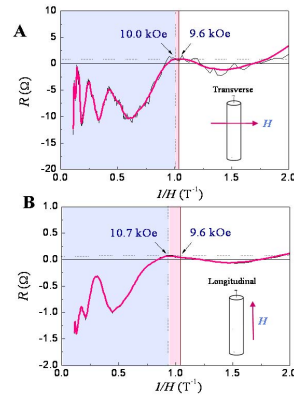
Fig. 2. SdH oscillations obtained by the external field of (A) transverse and (B) longitudinal to the wire axis.
