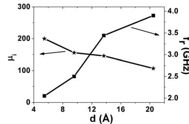
Fig. 1. The initial permeability \mu_i and resonance frequency f_r for the samples at various magnetic FeCoSi thicknesses d .
