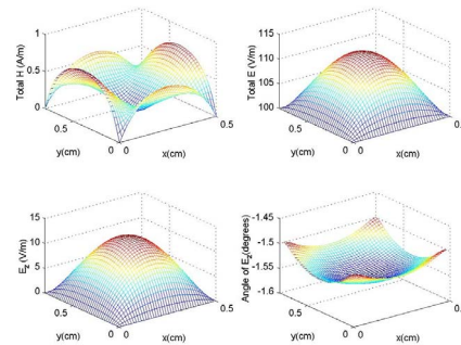
Fig. 1. Polarization enhancement.
