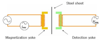
Fig. 1. Compose of magnetizing yoke and sensing yoke.
