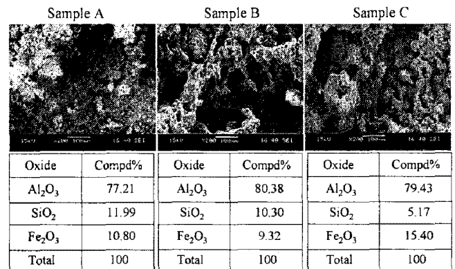
Fig. 6 SEM image and chemical composition of oxides
