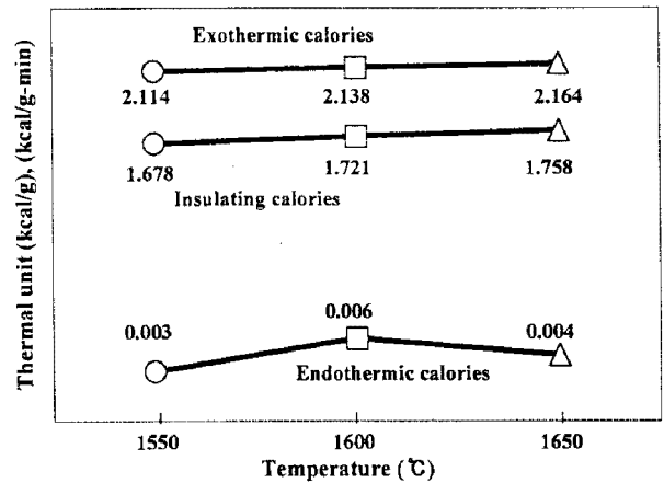
Fig. 4 Change of the thermal properties depending on the temperature
