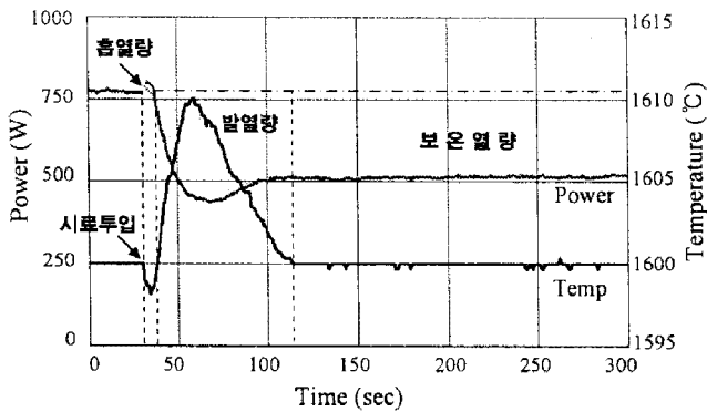
Fig. 3 Change of power and temperature depending on reaction time
