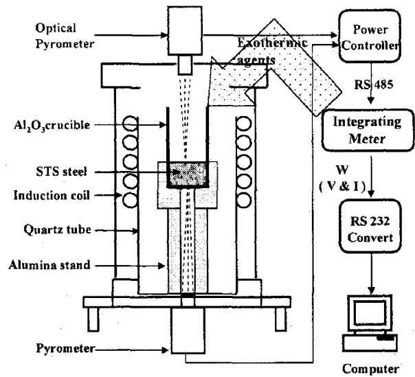
Fig. 2 Schematic drawing of experimental apparatus
