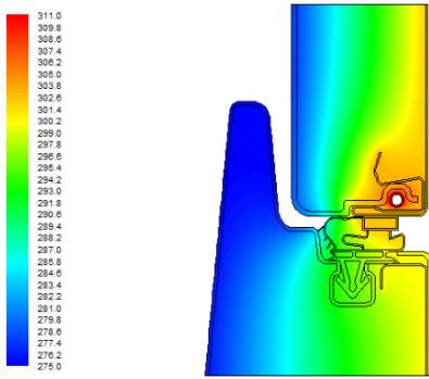
Fig. 5 Temperature contour of refrigerator side gasket region
