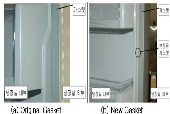
Fig. 4 Installed prototype gasket on the door of refrigerator
