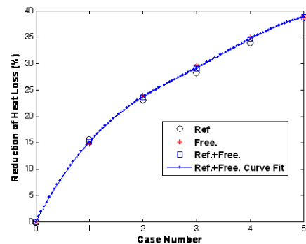
Fig. 8 Reduction of heat loss for the cases 0 to 5. o : refrigerator side, * : freezer side, □ : total reduction of heat loss.
