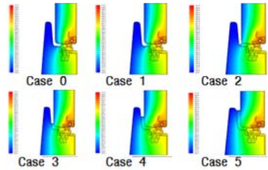
Fig. 7 Comparison of temperature contour with the variation of additional gasket position
