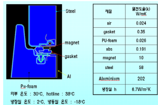
Fig. 2 Cross sectional view of refrigerator near gasket
