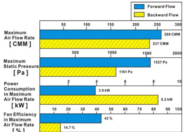
Fig. 12 Comparison of fan performance between forward flow and the backward flow.
