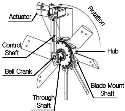
Fig. 2 Pitch angle Adjustment unit.
