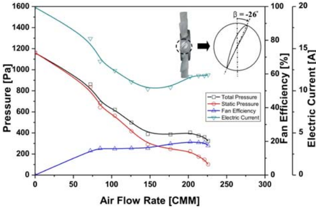
Fig. 8 Fan performance curve at -26^\circ pitch angle at backward flow situation.
