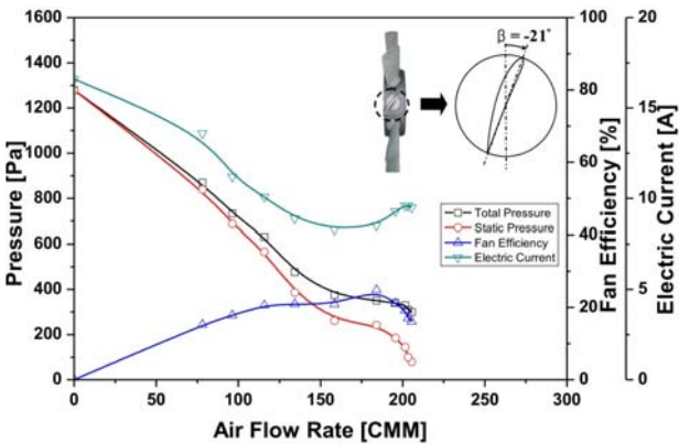
Fig. 9 Fan performance curve at -21^\circ pitch angle at backward flow situation.
