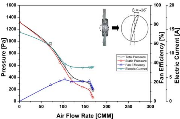
Fig. 10 Fan performance curve at -16^\circ pitch angle at backward flow situation.
