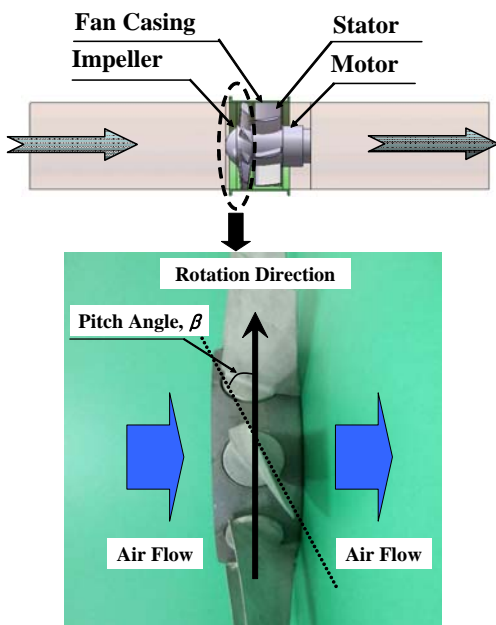
Fig. 3 Air flow direction and impeller shape at forward flow.
