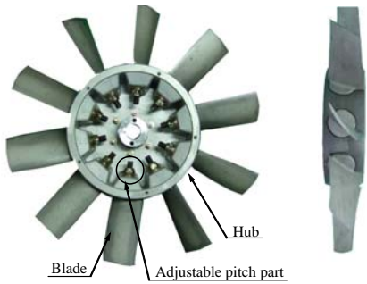
(a) Front view (b) Side view Fig. 1 Adjustable pitch angle impeller
