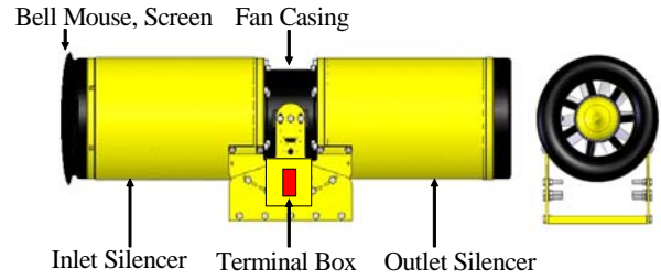
Fig. 5 Adjustable pitch axial fan in the present study.
