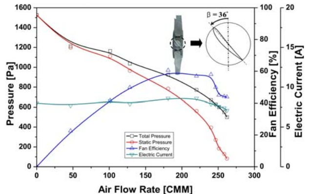
Fig. 7 Fan performance curve at 36° pitch angle at forward flow situation.
