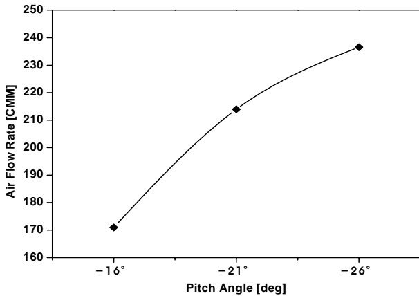
Fig. 11 Maximum air flow rate with pitch angle at backward flow situation.
