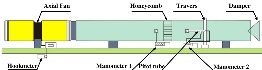
Fig. 6 Experimental equipment for a fan performance test.
