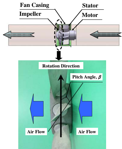
Fig. 4 Air flow direction and impeller shape at backward flow.
