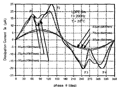
Fig. 1. Dissipation current waveforms obtained from different thickness film samples.
