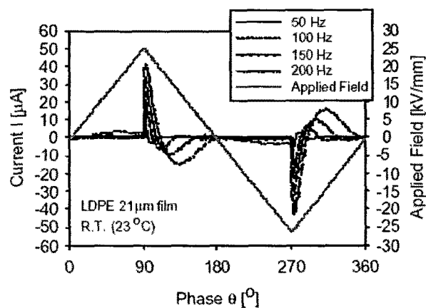
Fig. 3. Dissipation current waveform of LDPE film under triangle waveform application at each frequency.
