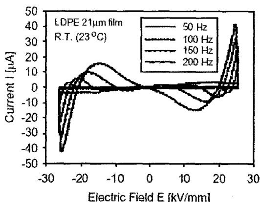
Fig. 4. E-I properties of LDPE film under triangle waveform application.
