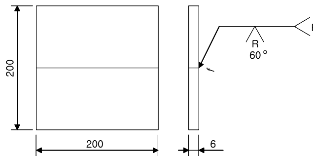
<Fig. 2> Welding size and method(unit:mm)
