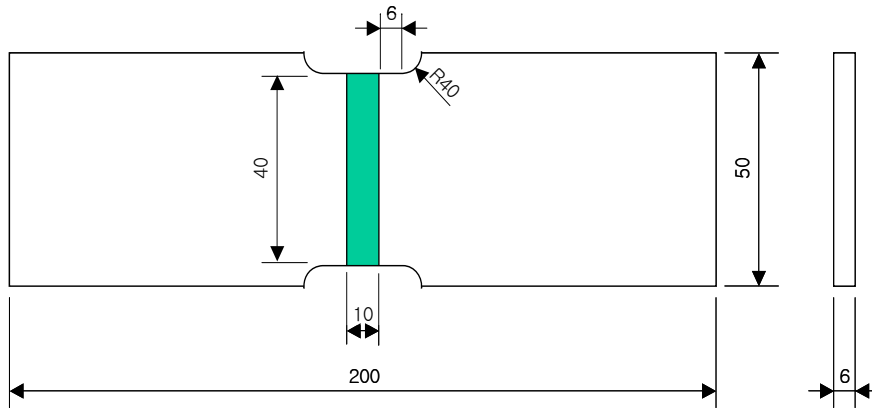
<Fig. 3> Geometry of test specimen(unit:mm)
