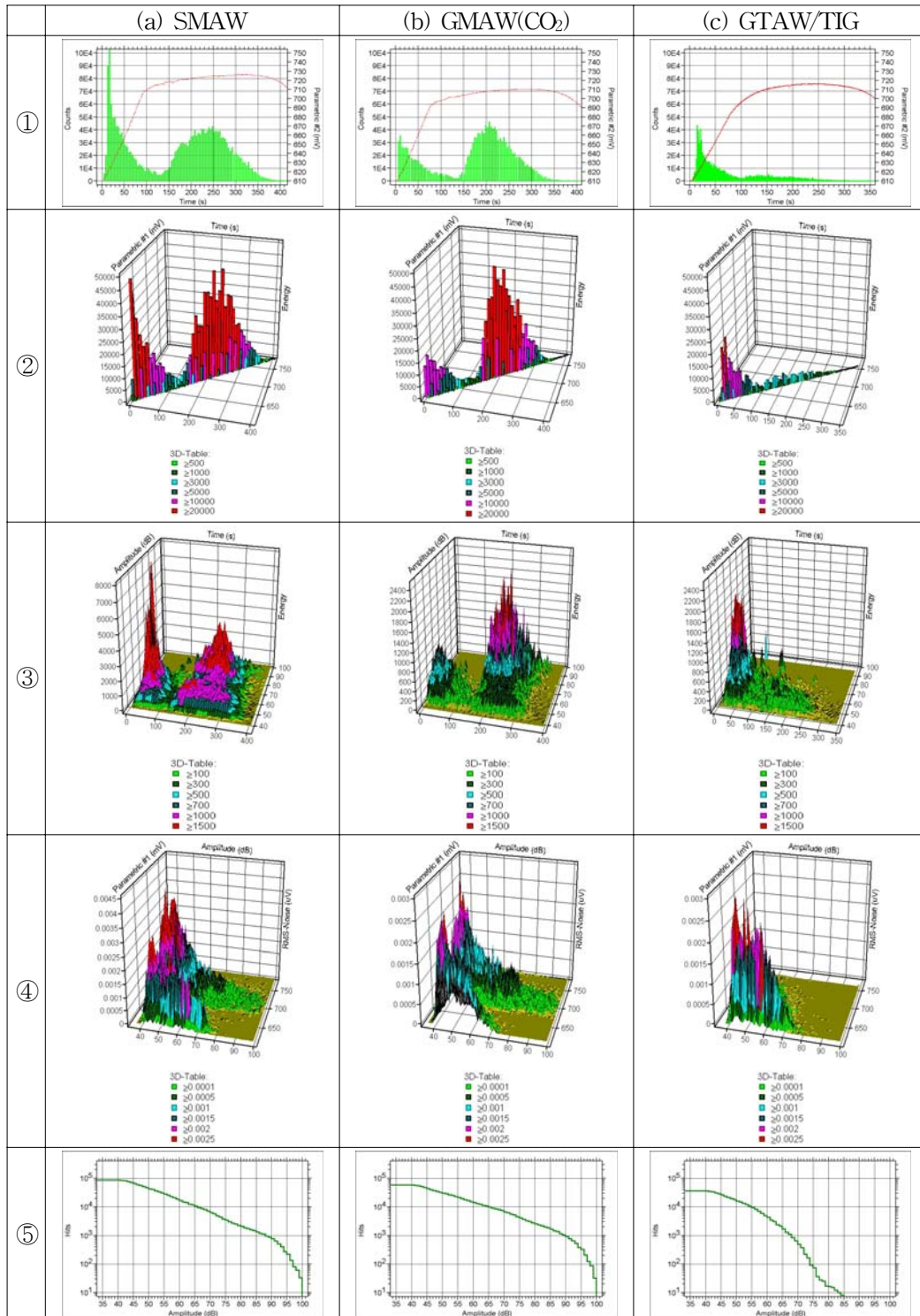
〈Fig. 4〉 Post-processing results of the detected AE signals
