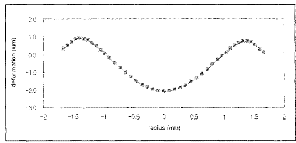
(a) CAE analysis result
