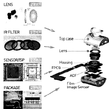
Fig. 1. Schematic description of an image sensing module
