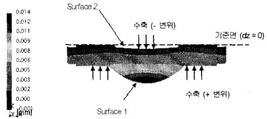
Fig. 4. Amount of deformation along the z-direction
