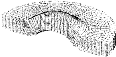
(b) mesh structure for the lens (2)
