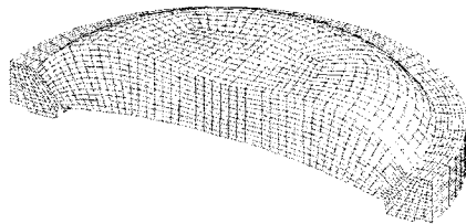
(c) mesh structure for the lens (3)
