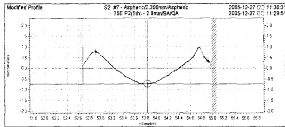
(b) Measured profile
