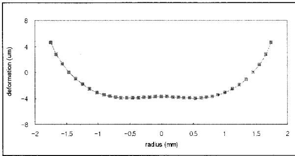
(a) CAE analysis result
