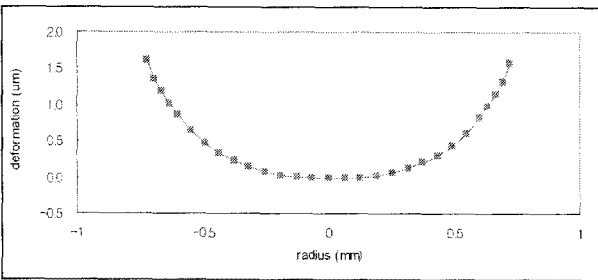
(a) CAE analysis result
