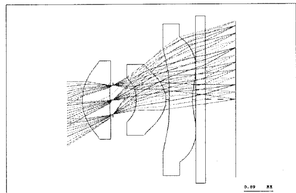
Fig. 2. Configuration of three aspheric lenses with ray tracing 7)
