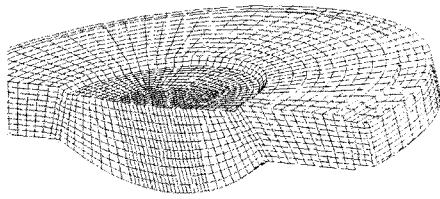
(a) mesh structure for the lens (1)
