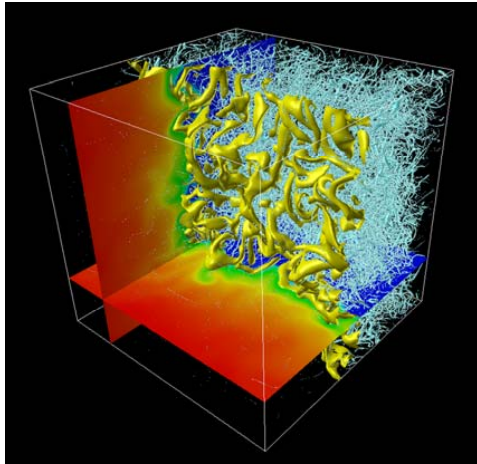
Fig. 1 Largest DNS of turbulent combustion in the world
