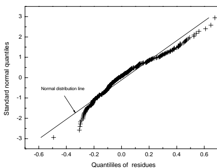
Fig. 8 Q-Q plot for residues
