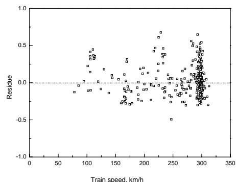
Fig. 9 Scatter plot for residues
