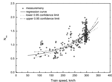
Fig. 7 Distributions of ride comfort indices and a regression curve
