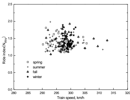
Fig. 6 Comparisons of Ride indices for seasons
