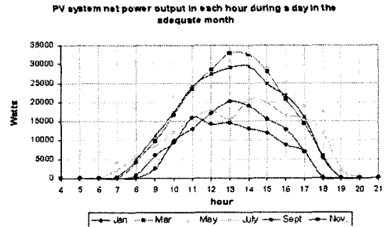
<Fig. 4> Generation Characteristic with monthly time variation
