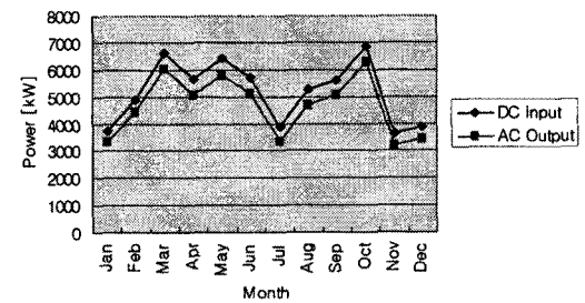
<Fig. 6> Monthly DC Input and AC Output of PCS
