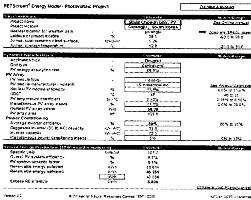
<Fig. 11> Energy Model of 50kW PV System
