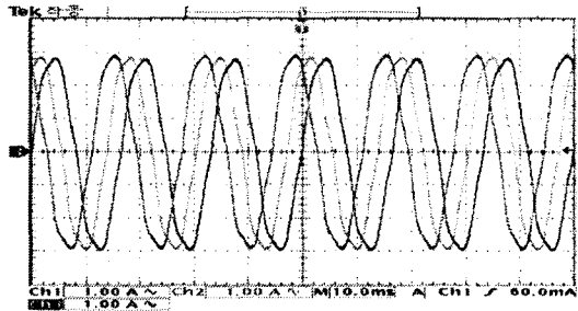
<Fig. 3> Inverter Current Waveforms with No Load
