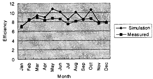
<Fig. 7> Monthly Generation Efficiency
