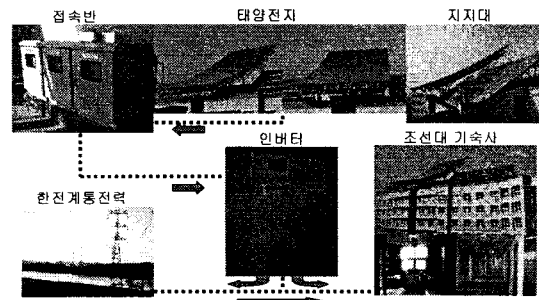
<Fig. 1> Overall System Configuration of the 50kW Grid Interconnected PV System
