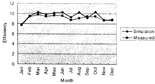
<Fig. 8> Monthly Array Conversion Efficiency
