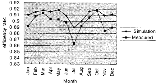
<Fig. 9> Monthly PCS Efficiency
