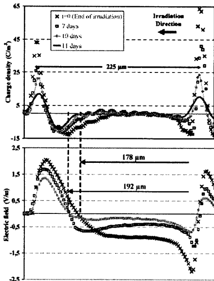
<Fig. 3> Kapton sample 225 \mu\text{m} -thick charge density recorded by PEA and electric field calculated during the relaxation after 30 min irradiation under 150 keV with a flux of 125 \text{pA}/\text{cm}^2 .
