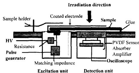
<Fig. 1> PEA Set-up for in-situ measurements.
