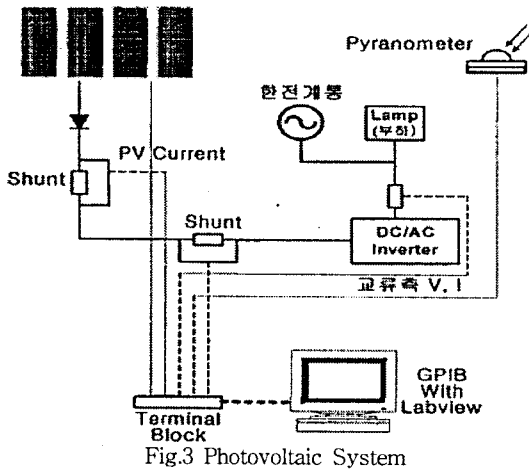
Fig.3 Photovoltaic System
