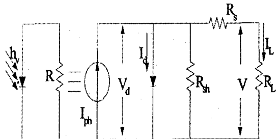
Fig.2 The equivalent circuit of solar cell
