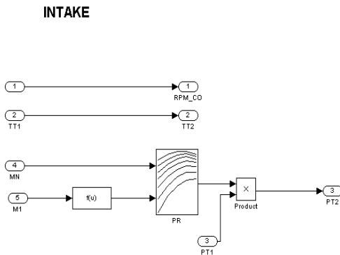
Fig. 3 Subsystem block of intake model
