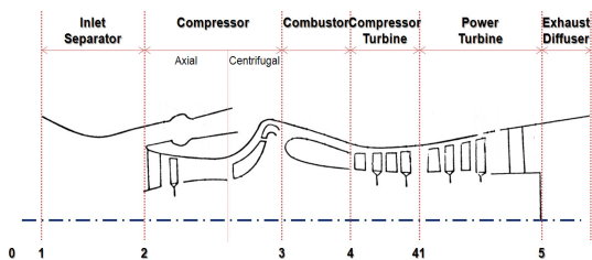
Fig. 1 Configurations and station numbering of the study engine
