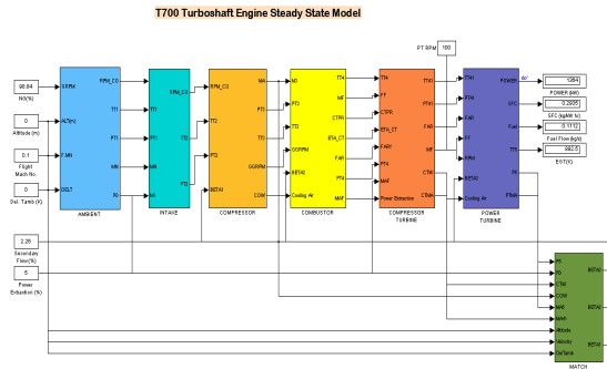
Fig. 2 Installed performance analysis modelling using SIMULINK
