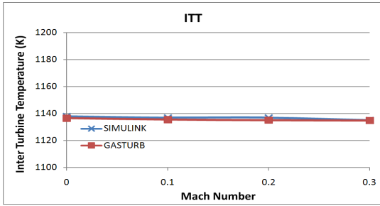
Fig. 4 Results of install performance analysis
