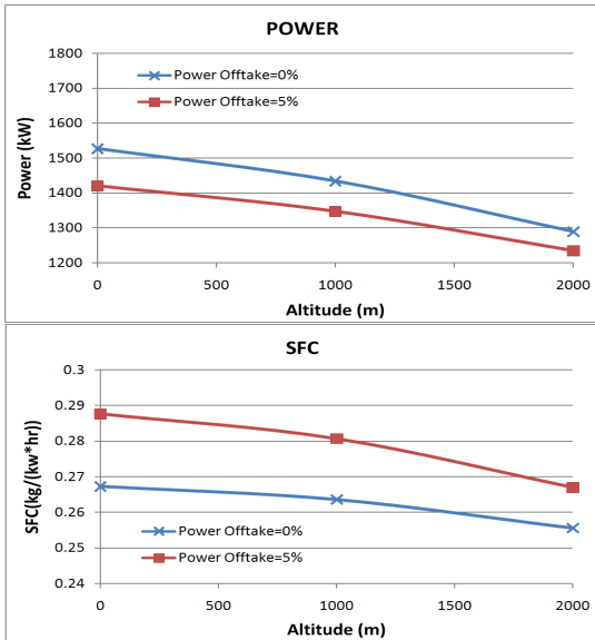
Fig. 5 Results of install performance analysis
