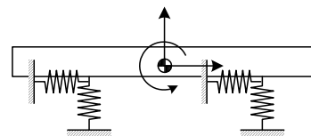
Fig. 5 Simplified model of a bearing system
