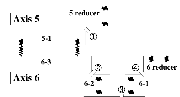
Fig. 4 Analytic model of a robot wrist
