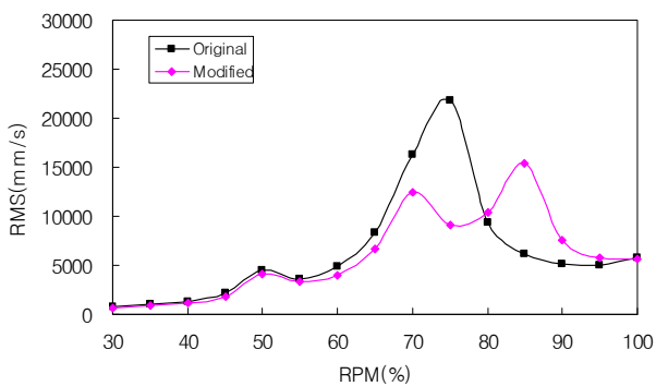
Fig. 8 Analysis result of an axial stiffness increase
