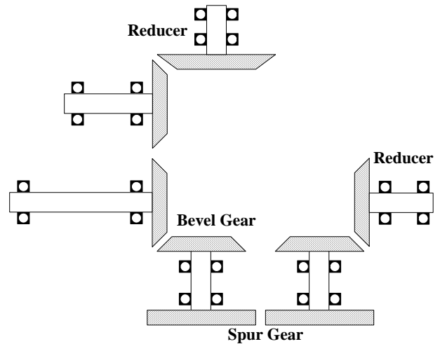
Fig. 2 Schematic diagram for axes 5 and 6
