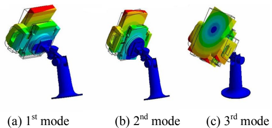
Fig. 10. Mode shapes of the existed car-holder
