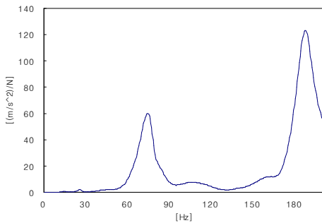
Fig.7. Frequency response function of the existed car-holder
