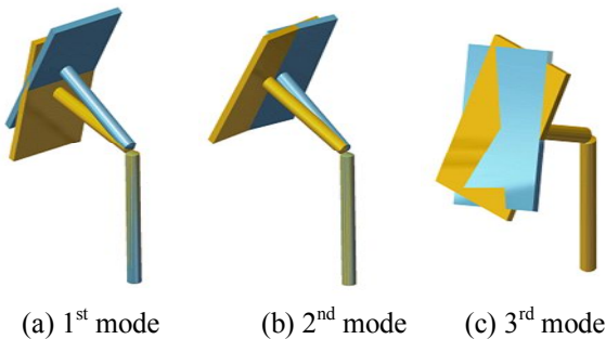
Fig. 8. Mode shapes of the existed car-holder
