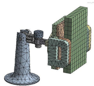
Fig. 9. Finite element model of the existed car-holder
