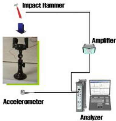
Fig. 6. Experimental setup for the modal testing
