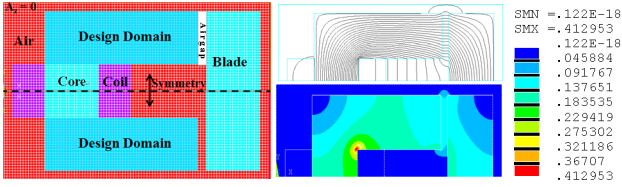
(a) Initial design (b) Magnetic flux line and Magnetic flux density
