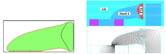
(a) Optimized level set design (b) FE reanalysis design <그림 6> Optimized C-core actuator and FEA result (steel and magnet)
