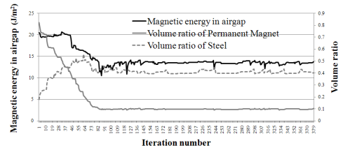
<그림 7> History diagram of Magnetic energy and volume ratio using steel and magnet
