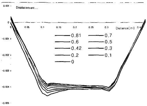
Fig. 6 Distribution of transverse distortions (At last step - Quarter Model)
