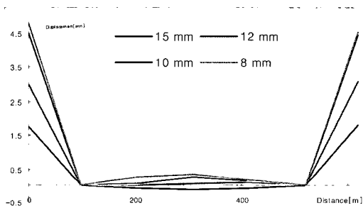
Fig. 8 Angular distortion of Test-piece
