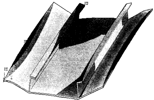
Fig. 3 Distortion simulation (At last step)
