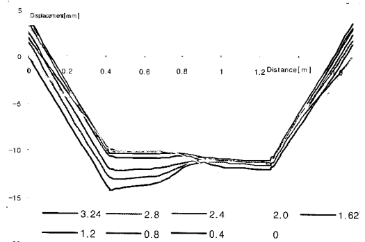
Fig. 4 Distribution of transverse distortions (At last step - Real Model)
