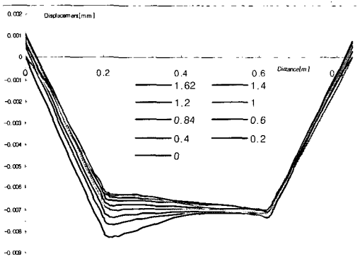
Fig. 5 Distribution of transverse distortions (At last step - Half Model)
