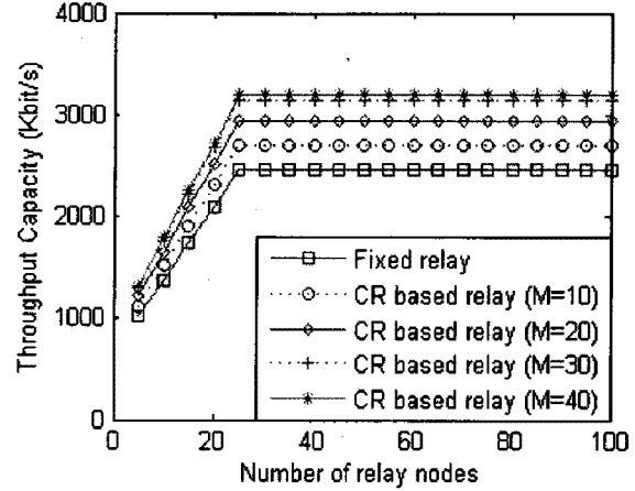
Fig.3. The throughput capacity of the proposed system varying number of CRs.
