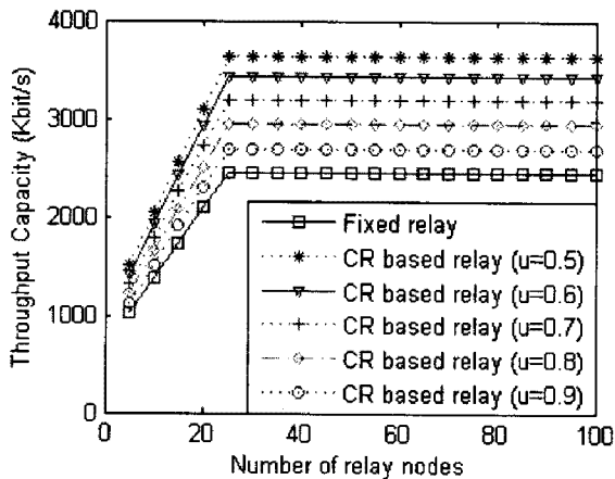
Fig.2. The throughput capacity of the proposed system varying utilization factor
