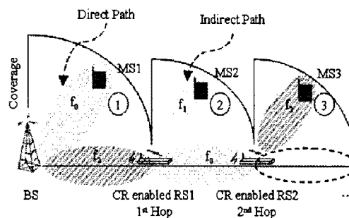
Fig.1. CR based Multi-hop cell architecture.
