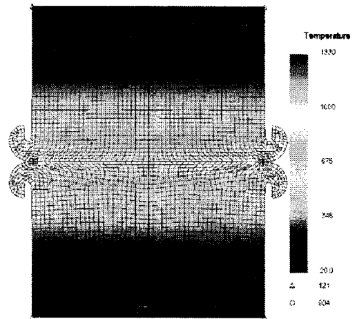
Fig. 3(b) Deformation shape and distribution of temperature after upset phase step
