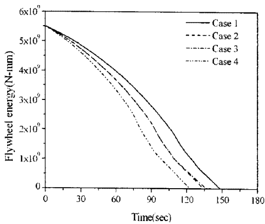
Fig. 2(a) Flywheel energy versus time curve
