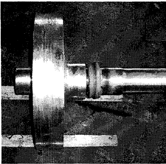
Fig. 4 Rotor shaft shape using friction welding
