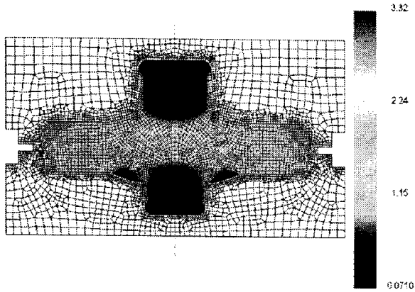
Fig. 1(a) Strain distribution and deformation shape after forging of flange part
