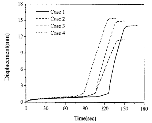
Fig. 2(b) Upset length versus time curve
