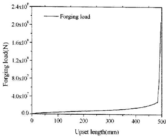
Fig. 1(b) Displacement versus forging load curve for closed die forging
