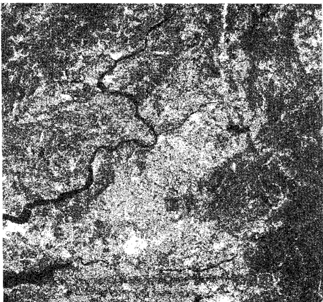
Figure 3. Coherence image (1998.07-08)
