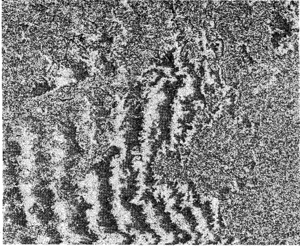
Figure 2. Interferogram image (1998.07-08)
