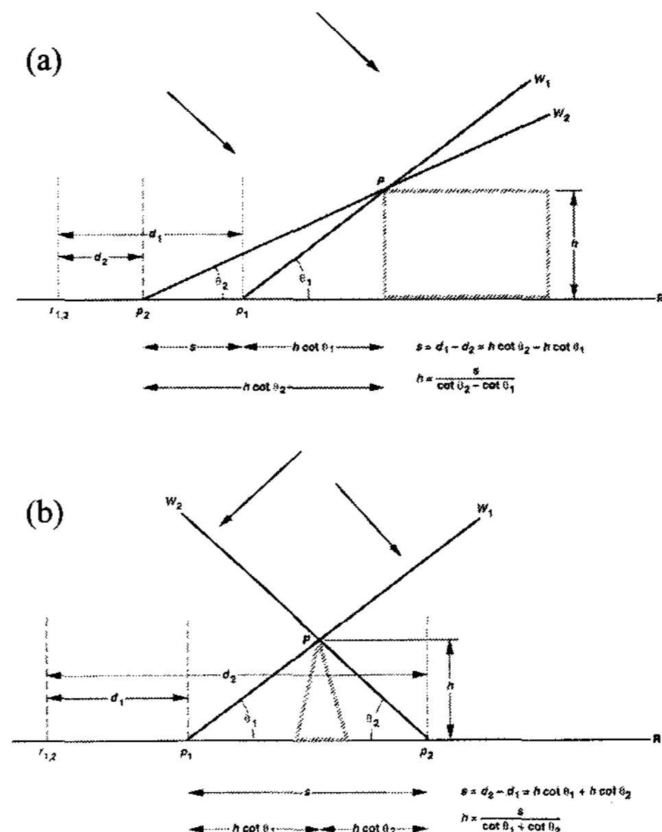
Figure 5. Geometries of radargrammetry of (a) same-side and (b) opposite-side (Ford et al. , 1993).
