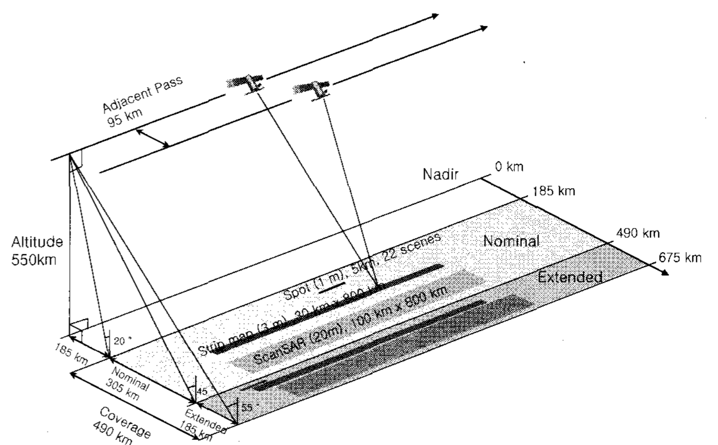
Figure 1. Imaging modes of KOMPSAT-5 SAR.
