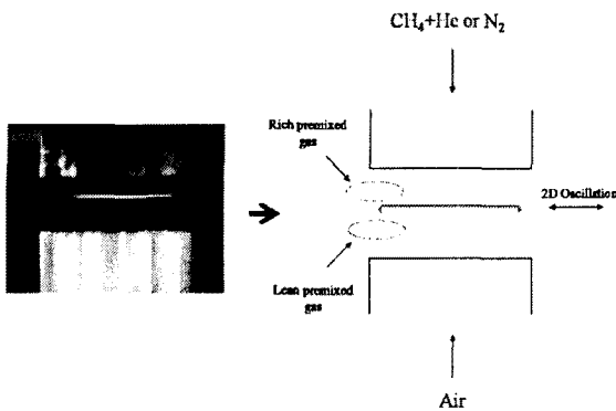
Fig. 1 Representative direct photo and schematic diagram of low strain rate counterflow flame configuration.
