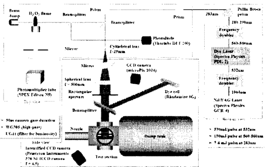
Fig. 2 OH-PLIF System
