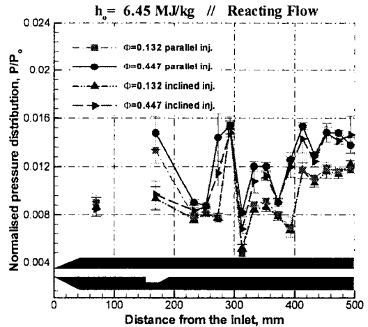
Fig. 8 Pressure Distribution Comparison of Reacting Flow between Parallel and Inclined Fuel Injection
