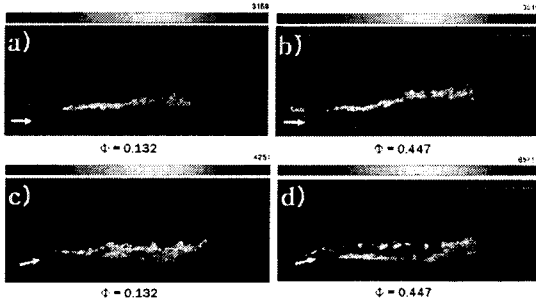
Fig. 6 OH-PLIF Comparison between Parallel and Inclined Fuel Injection
