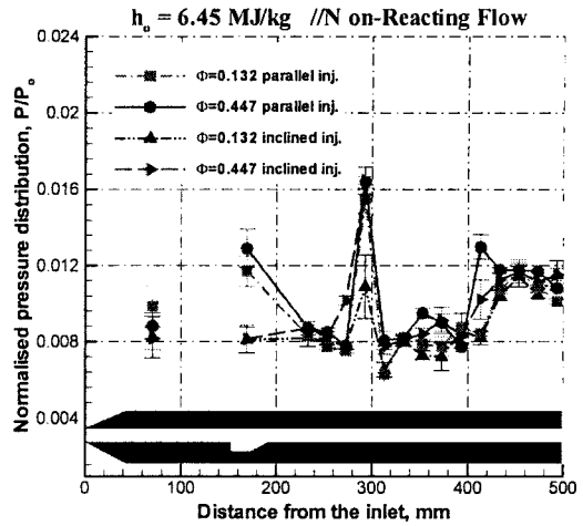
Fig. 7 Pressure Distribution Comparison of Non-Reacting Flow between Parallel and Inclined Fuel Injection
