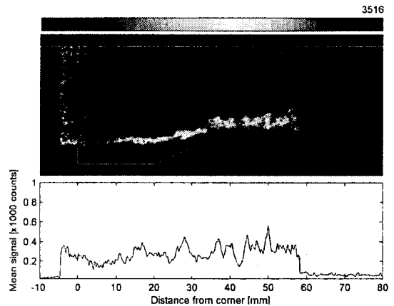
Fig. 4 OH-PLIF Image for \phi=0.447
