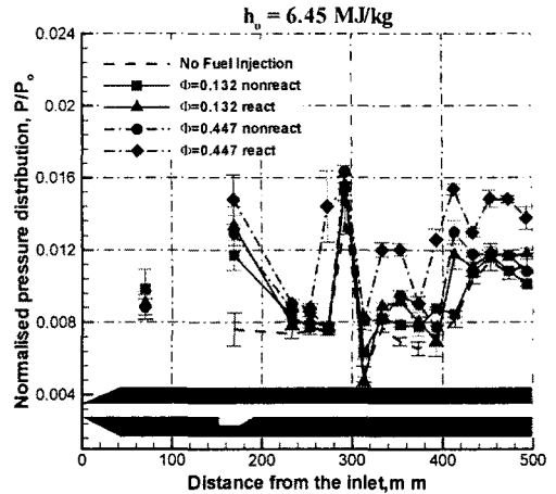
Fig. 5 Pressure Distribution in the Combustor for Parallel Fuel Injection
