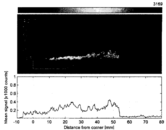
Fig. 3 OH-PLIF Image for \phi=0.132
