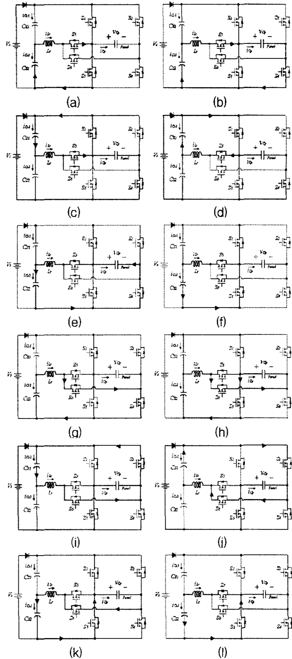
그림 2. 동작모드, (a)모드1, (b)모드2, (c)모드3, (d)모드4, (e)모드5, (f)모드6, (g)모드7, (h)모드8, (i)모드9, (j)모드10, (k)모드11, (l)모드12
