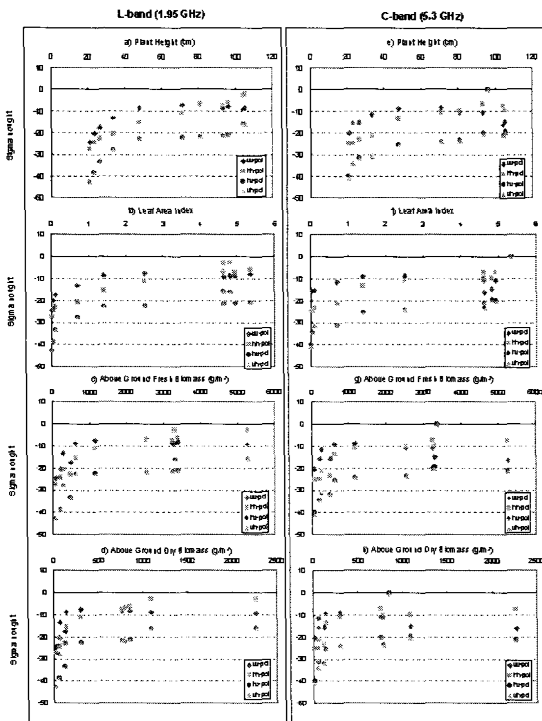
Fig. 2. Relationship between radar backscattering coefficients and rice growth at 50 degree incidence angle.
