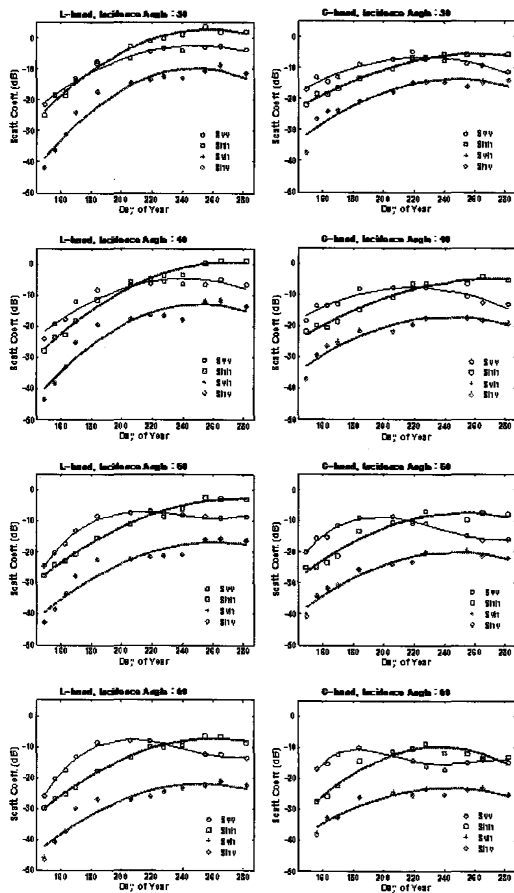
Fig. 1. Backscattering coefficients of rice growth as a function of time at different wavelengths, incidence angles, and polarization.
