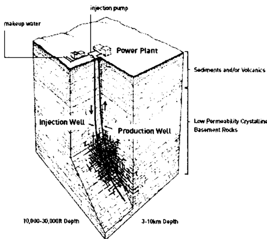
Figure 1. EGS의 개요 (Renewable Energy and Power Department, 2006)
