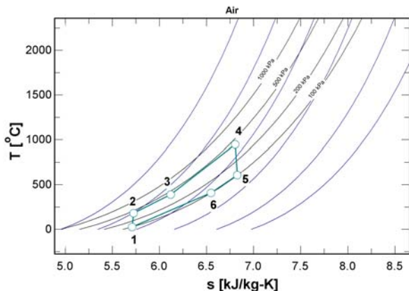
Fig. 2 T-s diagram for 60 kW microturbine
