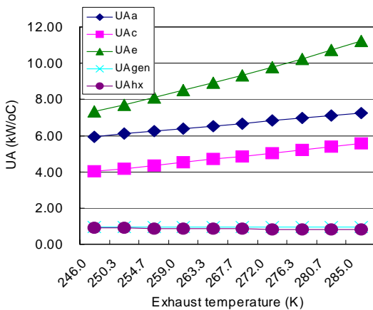
Fig. 7 Effects of exhaust temperature on the overall heat transfer coefficient of the heat exchangers of absorption chiller.
