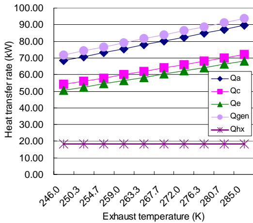
Fig. 6 Effects of exhaust temperature on the heat transfer rate of the heat exchangers of absorption chiller.
