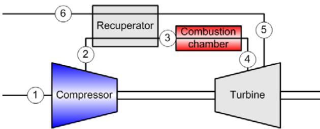
Fig. 1 Schematic of microturbine
