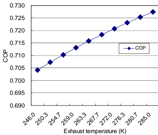
Fig. 8 Effects of exhaust temperature on the COP of absorption chiller.
