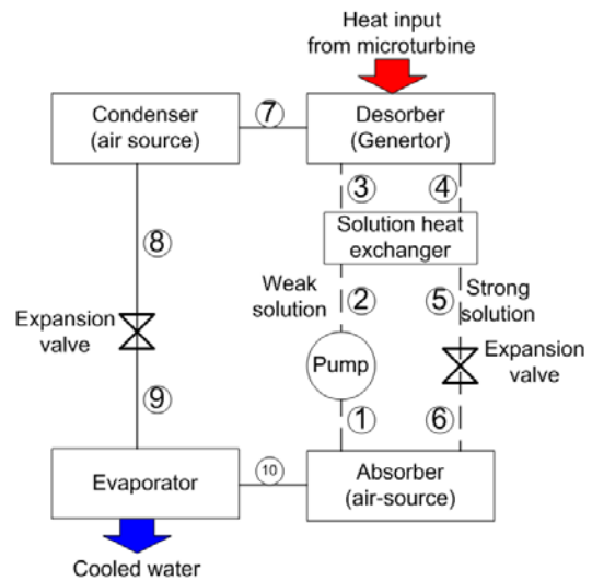
Fig. 3 Schematic of absorption chiller
