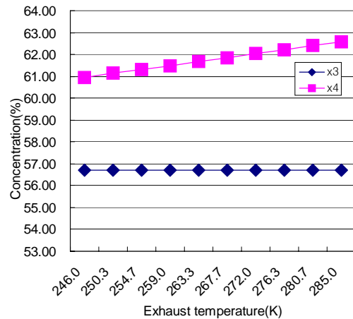
Fig. 4 Effects of exhaust temperature on the concentration of LiBr solution of absorption chiller.
