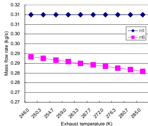
Fig. 5 Effects of exhaust temperature on the mass flow rate of the LiBr solution of absorption chiller.
