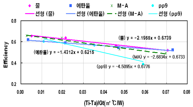
Fig 12. Collector angle 60°
