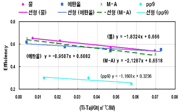
Fig 10. Collector angle 20°
