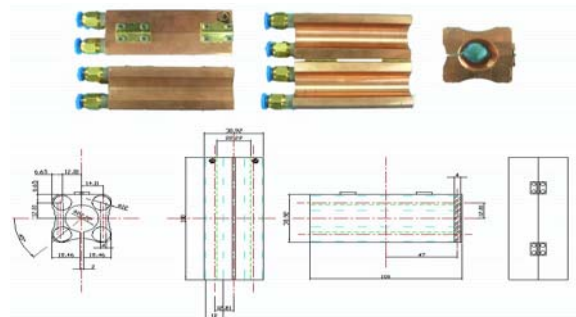
Fig 5. Manifold
