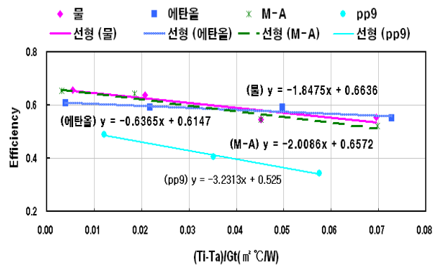
Fig 11. Collector angle 40°
