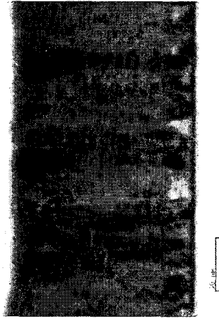
Fig. 1. Cross-sectional TEM image for Co 3 Pt electroplated on the Ru buffer.
