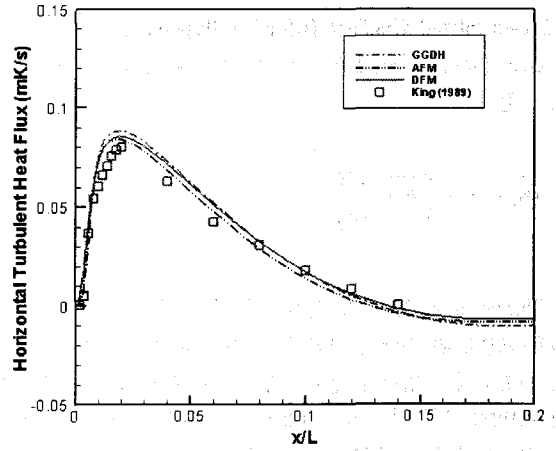
(a) Horizontal turbulent heat flux
