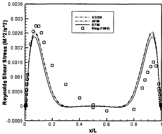
Fig.3 Reynolds shear stress profiles at y/H=0.5.
