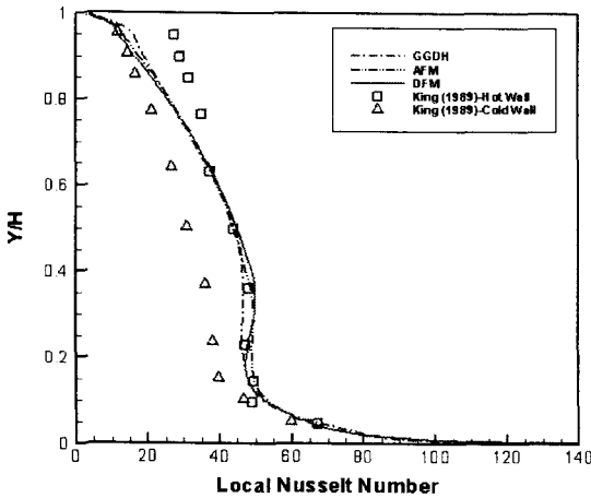
Fig.6 Local Nusselt number along the hot wall
