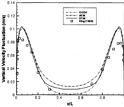
Fig.2 Vertical velocity fluctuation profiles at y/H=0.5
