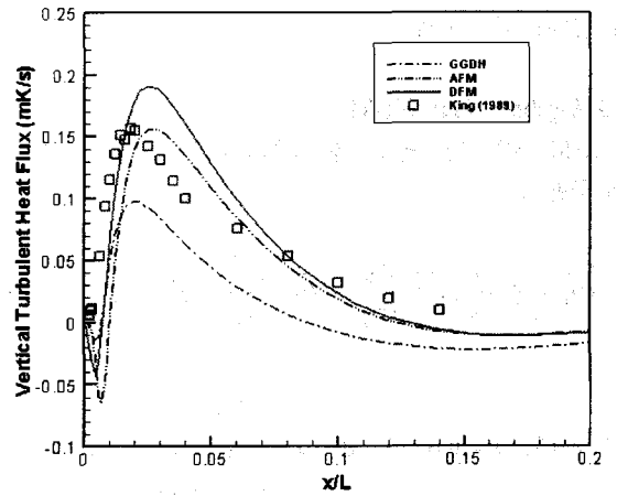
(a) Vertical turbulent heat flux
