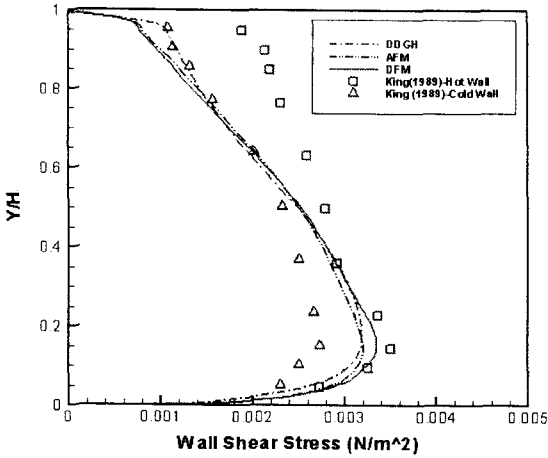
Fig.5 Wall shear stress profile along the hot wall
