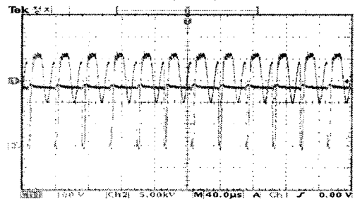
Figure 7 . High tension output (430V), coil both end output (12 K V),(433V)
