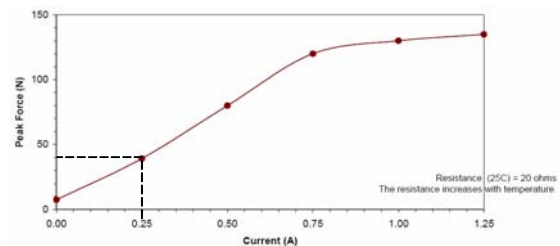
Fig. 3 Peak force and current of the MR damper
