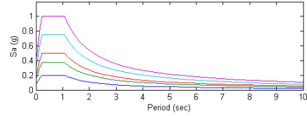
(b) C_V/C_A = 2.67
