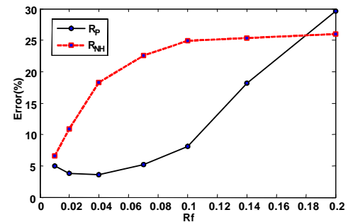
Fig. 7 Maximum peak displacement errors with respect to the normalized friction force
