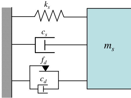
Fig. 1 SDOF system with MR damper
