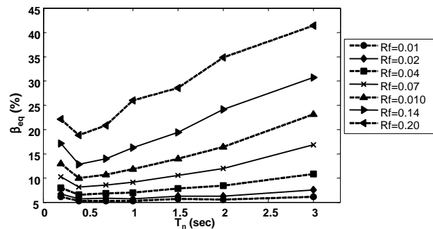
(b) C_V/C_A = 2.67
