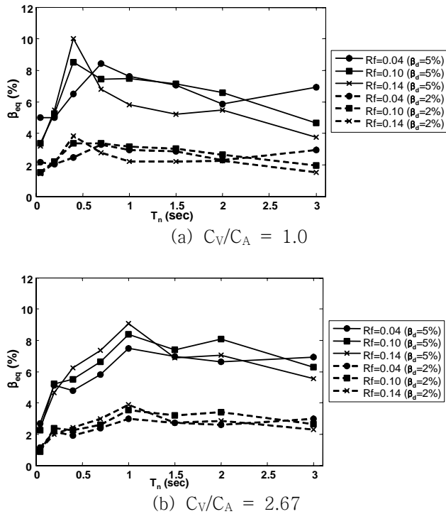
Fig. 10 Increment of equivalent damping ratio by the viscous damping in the MR damper ( C_V=0.08 )
