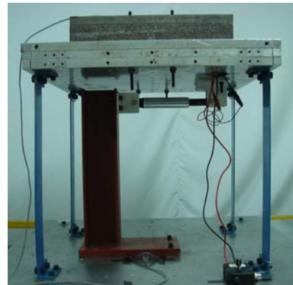
Fig. 2 Setup of a SDOF with the MR damper
