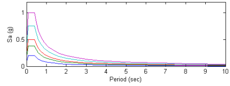
(a) C_V/C_A = 1.0
