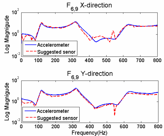
Fig. 6 Comparison of FRF's measured by the suggested sensor and an accelerometer at \theta = 45^\circ .
