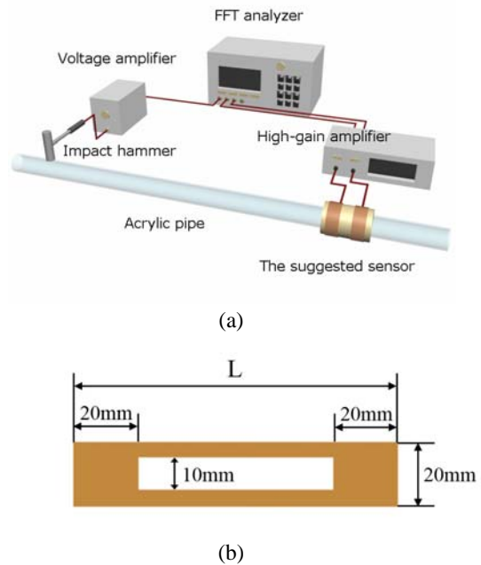
Fig.4 (a) Schematic illustration of the experiment setting for modal testing using the suggested sensor, (b) The shape of copper foil patches.
