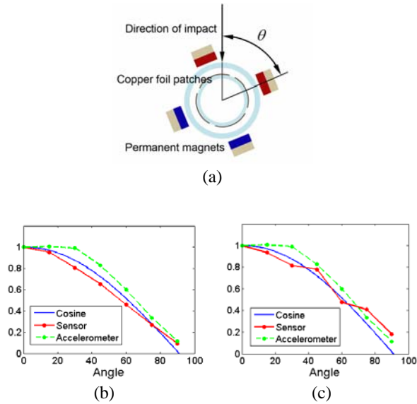
Fig.5 (a) Schematic diagram for the measurement of vibration in arbitrary direction, (b) Normalized sensitivity of the suggested sensor(L=150mm patch) for varying excitation angles measured in x-direction, (c) y-direction.
