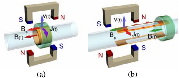
Fig.1 (a) Illustration of the working principle of the sensor suggested by Han and Kim at acrylic pipe (7) , (b) Illustration of the working principle-remote sensing- of the suggested sensor.
