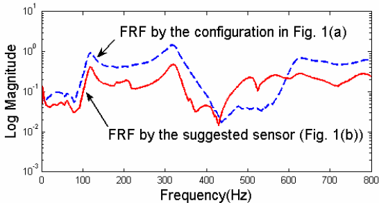
Fig.2 FRF plots in each sensor's configuration
