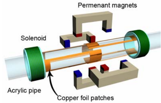
Fig.3 Illustration of the sensor to measure bending vibration in two orthogonal axis.
