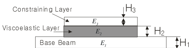
Figure 1. Constrained damping layer beam.
