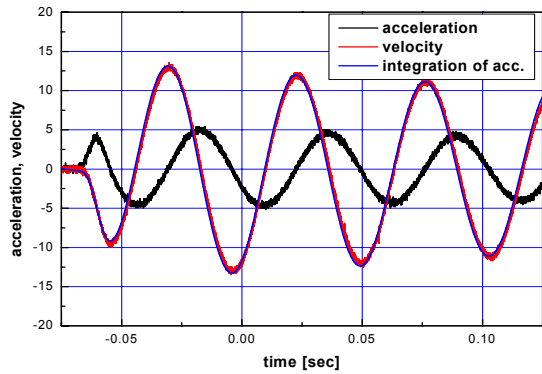
Fig. 10 Vibration signals of low frequency ranges after DC offset compensation.
