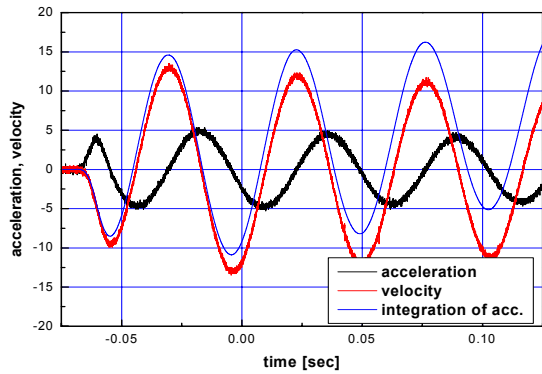
Fig. 9 Vibration signals of low frequency ranges before DC offset compensation.
