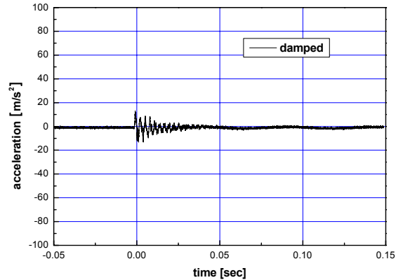
Fig. 8 Vibrational signals of high frequency ranges with mechanical filter
