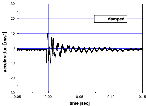
Fig. 7 Vibrational signals of middle frequency ranges with mechanical filter
