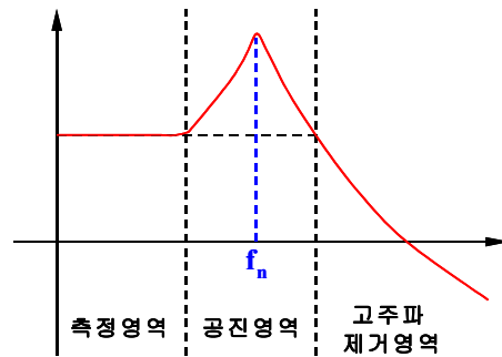
Fig. 3 General vibrational signal ranges
