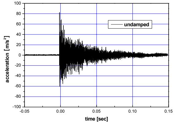
Fig. 7 Vibrational signals of high frequency ranges without mechanical filter
