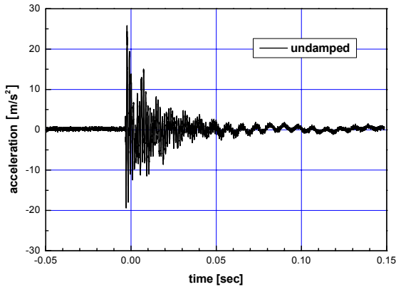
Fig. 5 Vibrational signals of middle frequency ranges without mechanical filter
