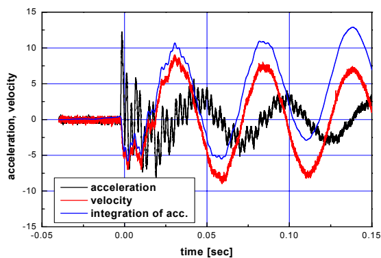
Fig. 11 Vibration signals of high frequency ranges before DC offset compensation.
