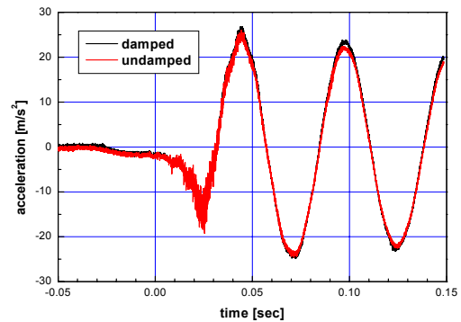
Fig. 4 Difference of vibrational signals with and without mechanical filter
