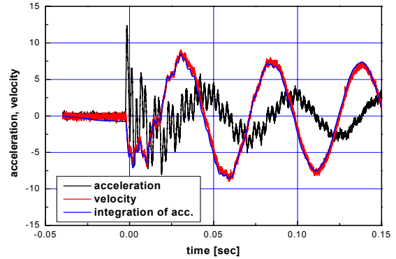
Fig. 12 Vibration signals of high frequency ranges after DC offset compensation.
