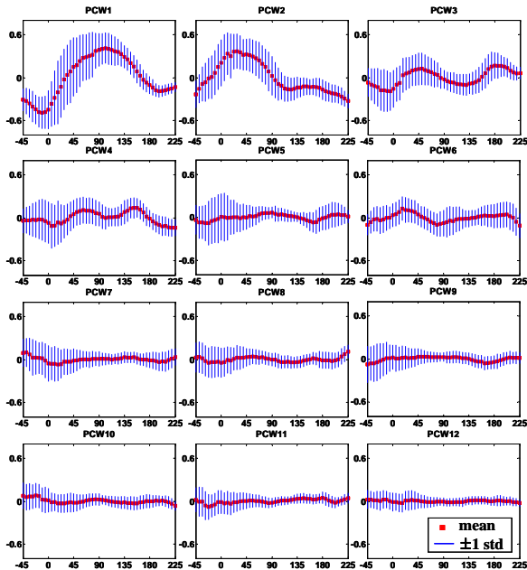
Fig. 5. Mean and \pm 1 standard deviation of each PCW for all left ear HRIRs (45 subjects) with respect to the change of median source elevation.
