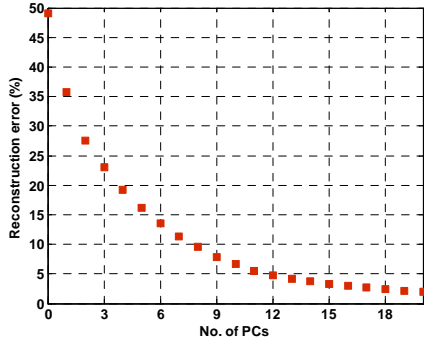
Fig. 2. Reconstruction errors with respect to the number of PCs
