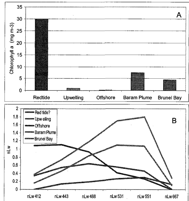
Figure 3. MODIS Aqua chl-a (A) and nLw spectral (B) for upwelling region, off shore water, Baram River plume, Brunei Bay and potential red tide area.
