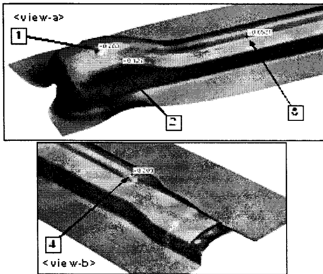
Fig. 3 (a) SP782-390 1.8t - Thickness reduction
