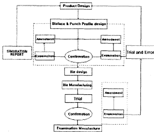
Fig. 1 Flow chart for die manufacturing
