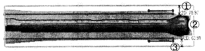
Fig. 4 (b) Metal Flow
