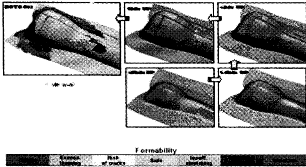
Fig. 2 (b) SP781-590 1.6t - Wrinkling
