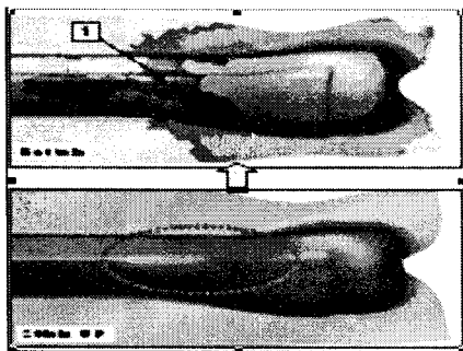
Fig. 3 (b) SP782-390 1.8t - Wrinkling
