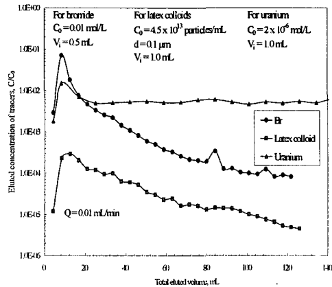
Fig. 2. Interim results for the nuclide migration experiments.
