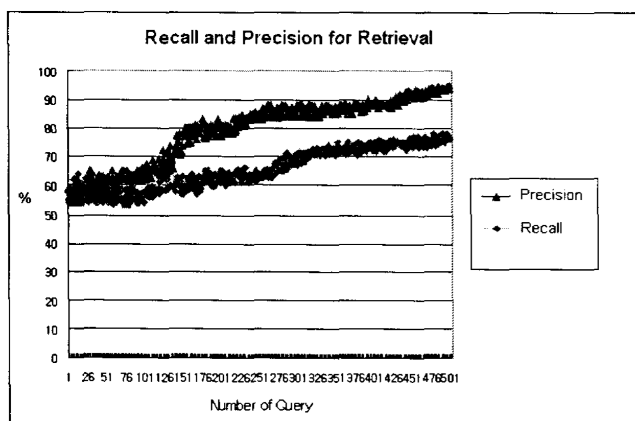
Fig 3. Retrieval Recall & Precision of the Proposed System
