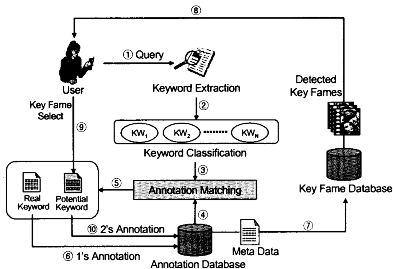
Figure 1. Automatic Annotation Processing
