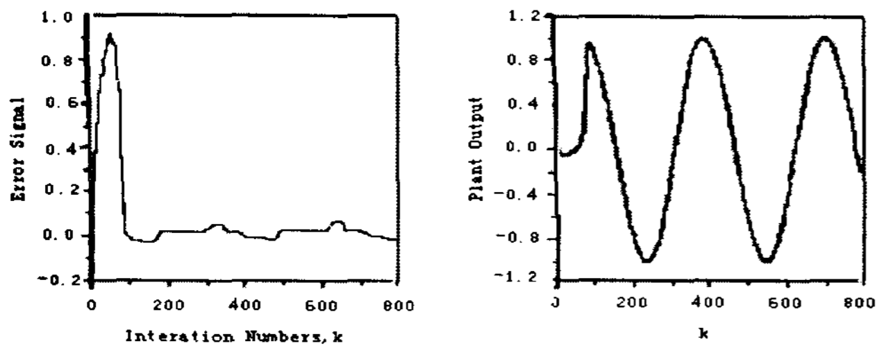
Fig 6. Error Signal of typical DNN
