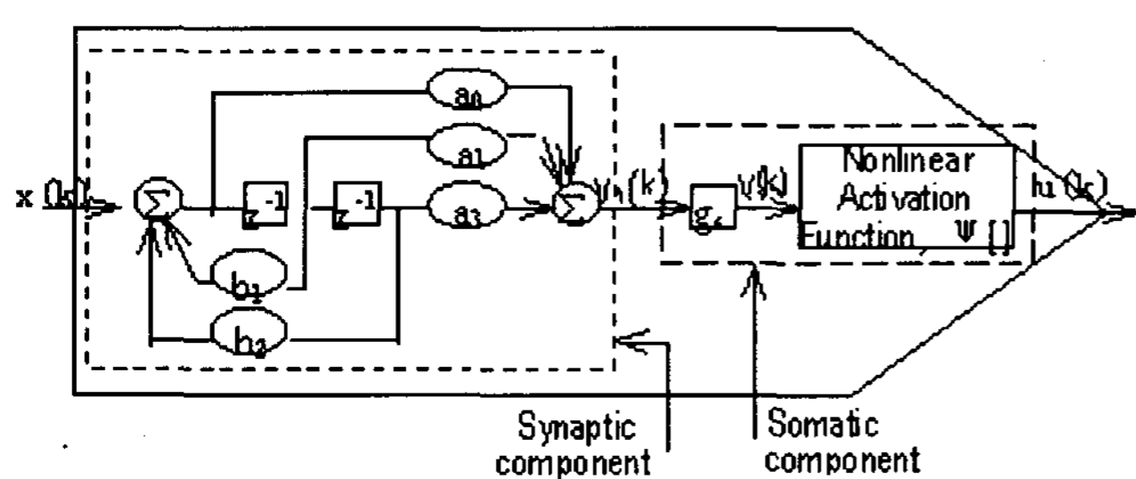
Fig 1. Basic structure of DNU, which consists of synaptic and somatic components.
