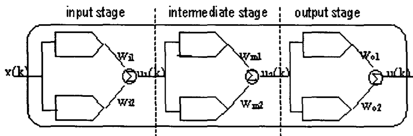
Fig 4. the Dynamic Neural Network structure
