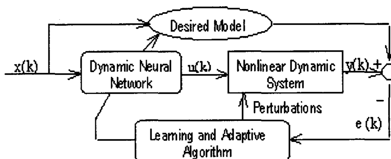
Figure 3. Control scheme for a nonlinear dynamic system using dynamic neural network
