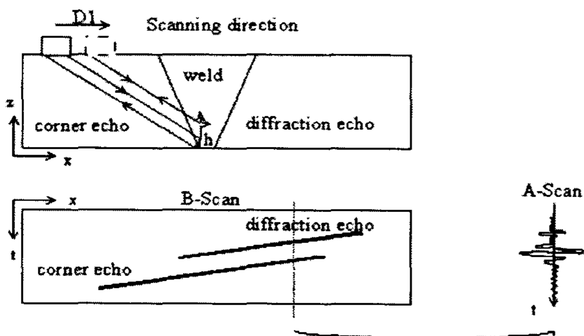
Fig 1. Ultrasonic Examination
